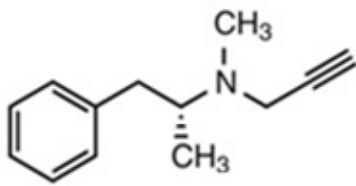
Selegiline
