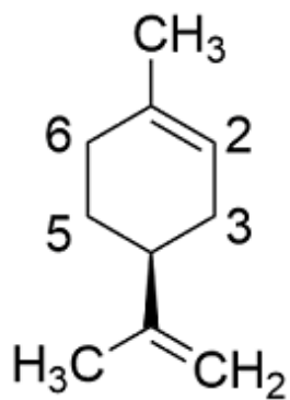
(-)- (4S)- limonene
