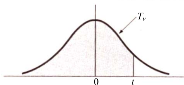
T DISTRIBUTION
