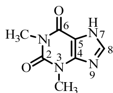
Theophylline
