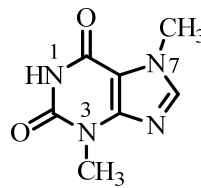
Theobromine
